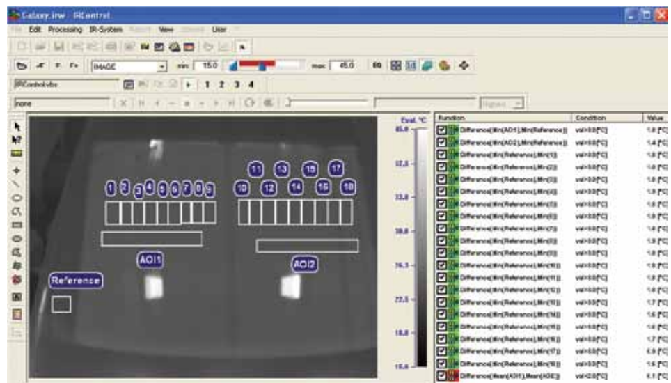
The control system Rato supplied for the rear window cannot be used here. Instead, the FLIR A320 records the maximum and minimum temperatures within the designated squares and the PLC compares these readings with previously determined parameters.
