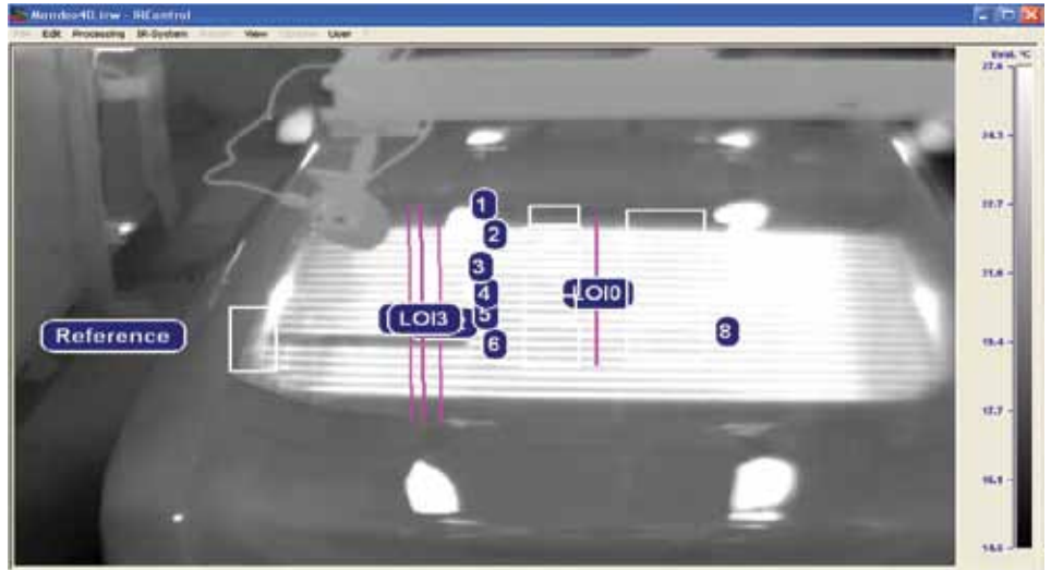
The special software tool that Rato supplied Ford Genk with compares the temperature measurements the FLIR A320 thermal imaging camera made along the purple lines.
