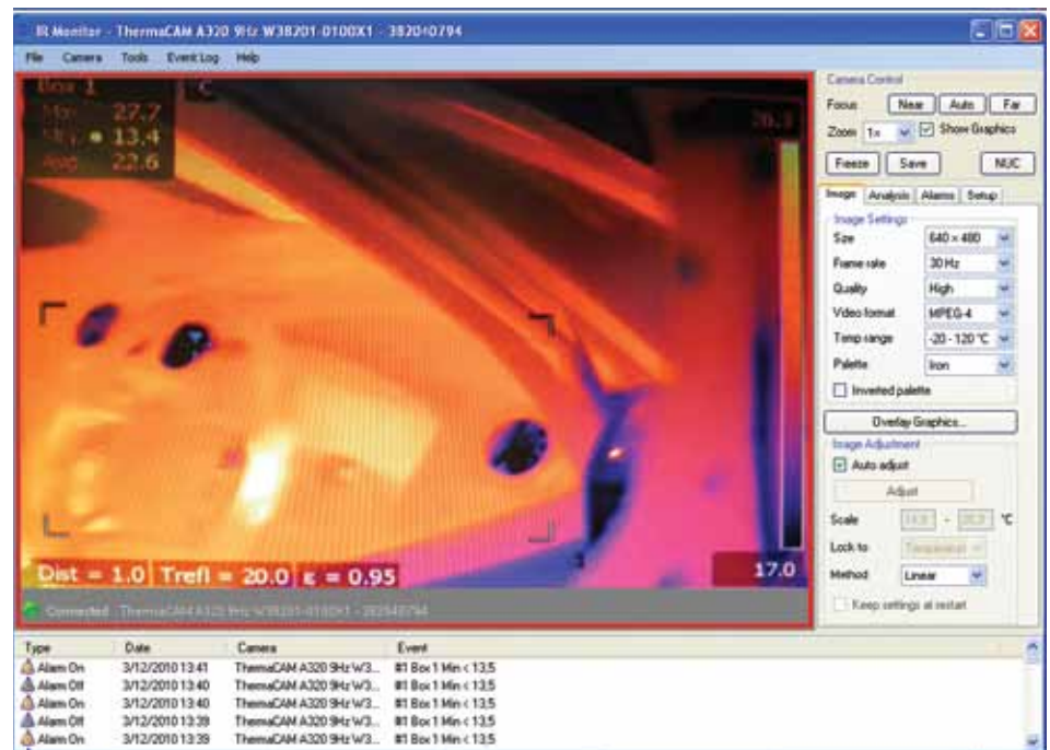
The temperature of the air coming out of the air conditioning vent that the FLIR A320 has recorded is sent to the PLC for comparison with previously determined parameters.
